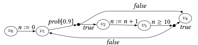
Figure 6. Control-flow hyper-graph of the program in Ex. 3.4
